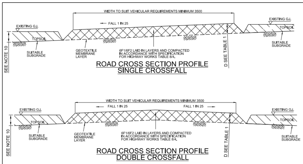
Plate 2.12: Typical Access Track Cross Section (solid ground)
