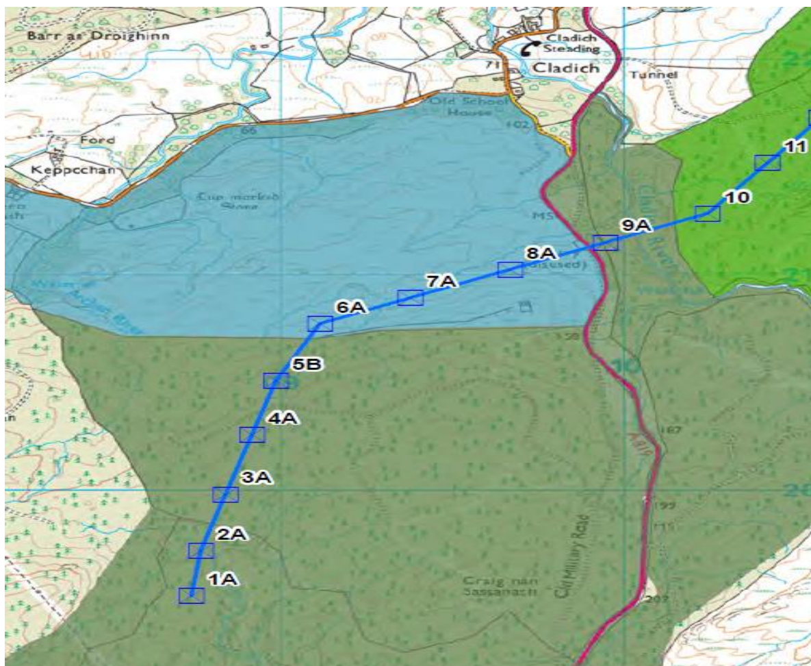
Plate 4.1: OHL T1 to T10
