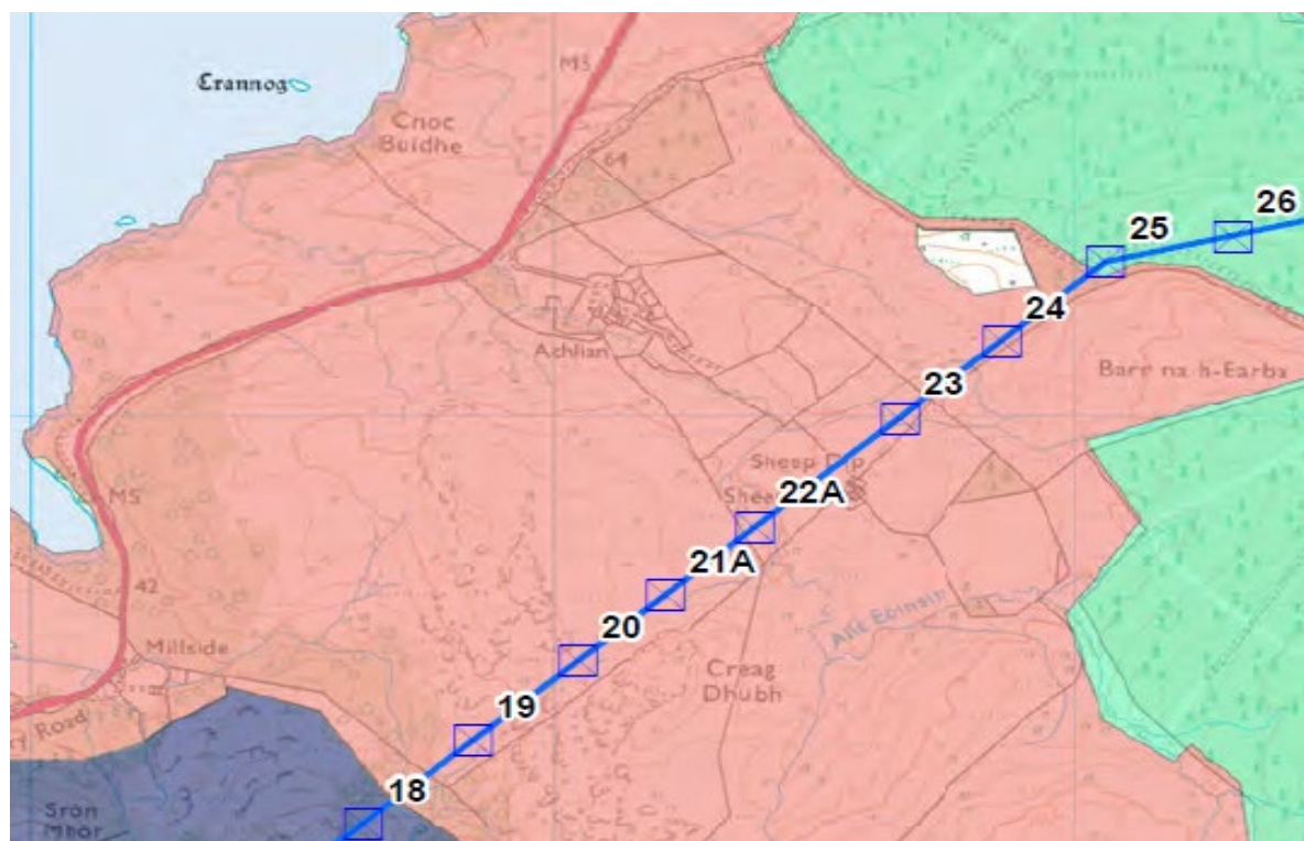
Plate 4.2: OHL T18 to T25
