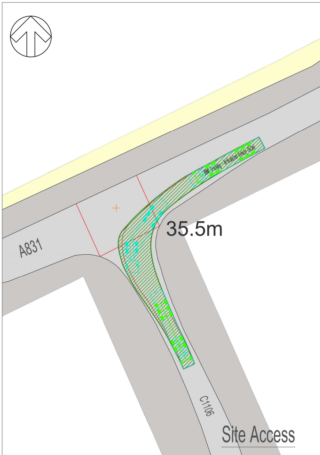
Figure 13.1.7.2: Potential Constraint at A831 / C1106 Junction
