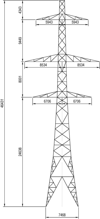
NEW LINE L8(c) D SUSPENSION TOWER
