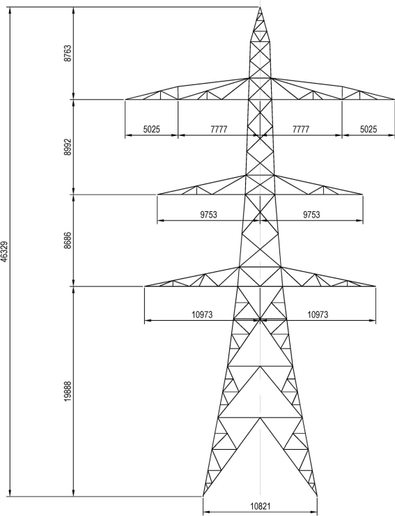
NEW LINE L8(c) DT TOWER
