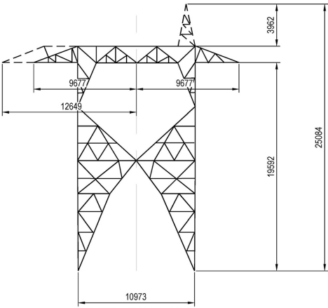
NEW LINE L8(c) SF60 TOWER
