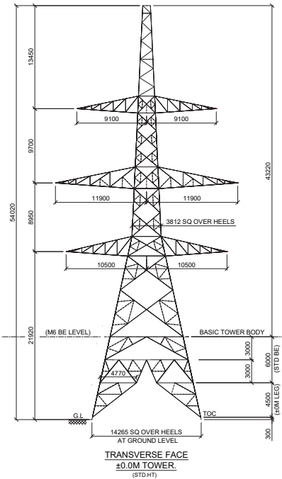
CONCEPTUAL KEY DIAGRAM FOR AS4 AD25 TYPE TOWER (10-25 DEG)
