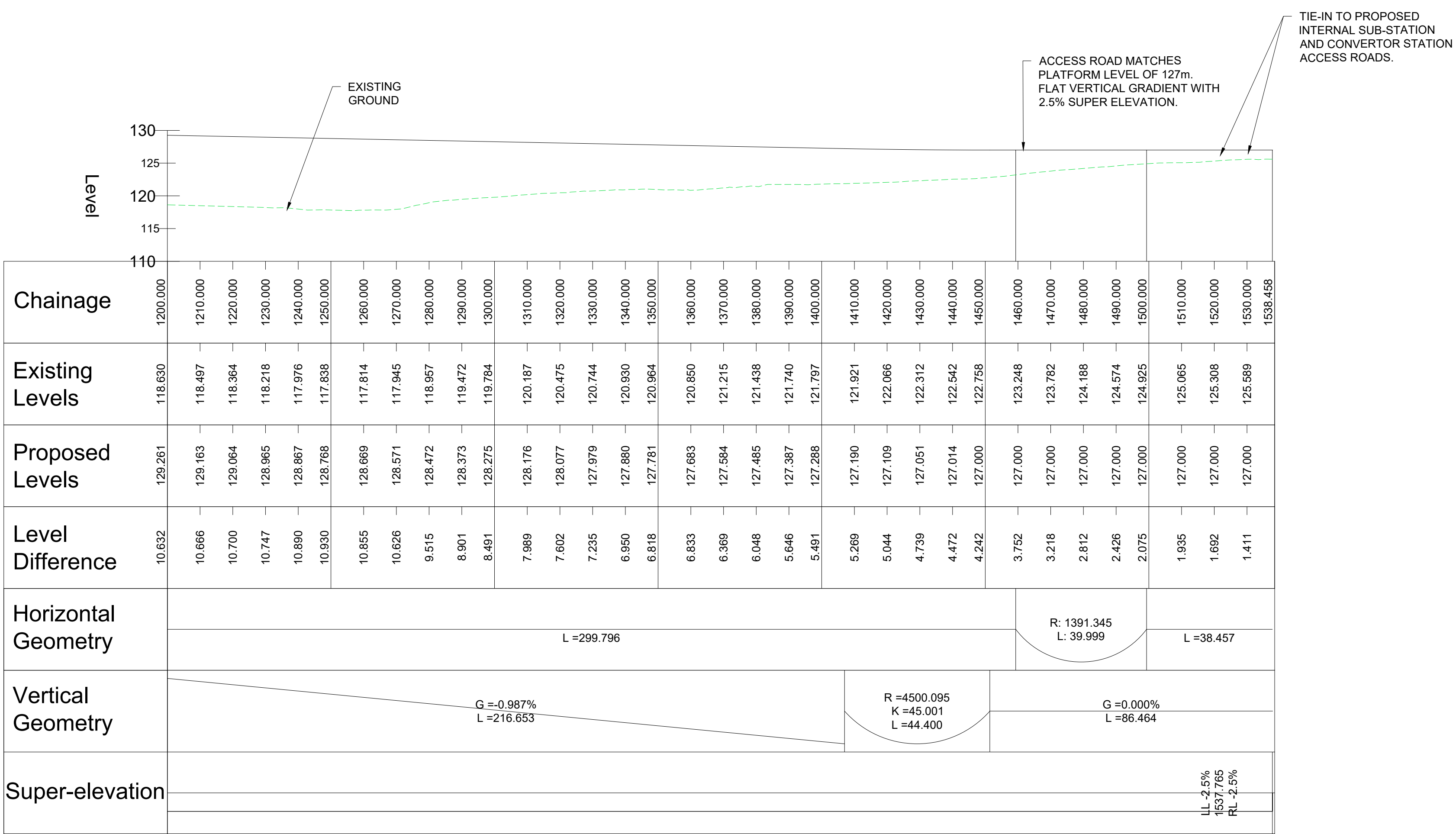
PERMANENT ACCESS ROAD PROFILE 1200-1538m SCALE 1:1000 HORIZONTAL, 1:500 VERTICAL
