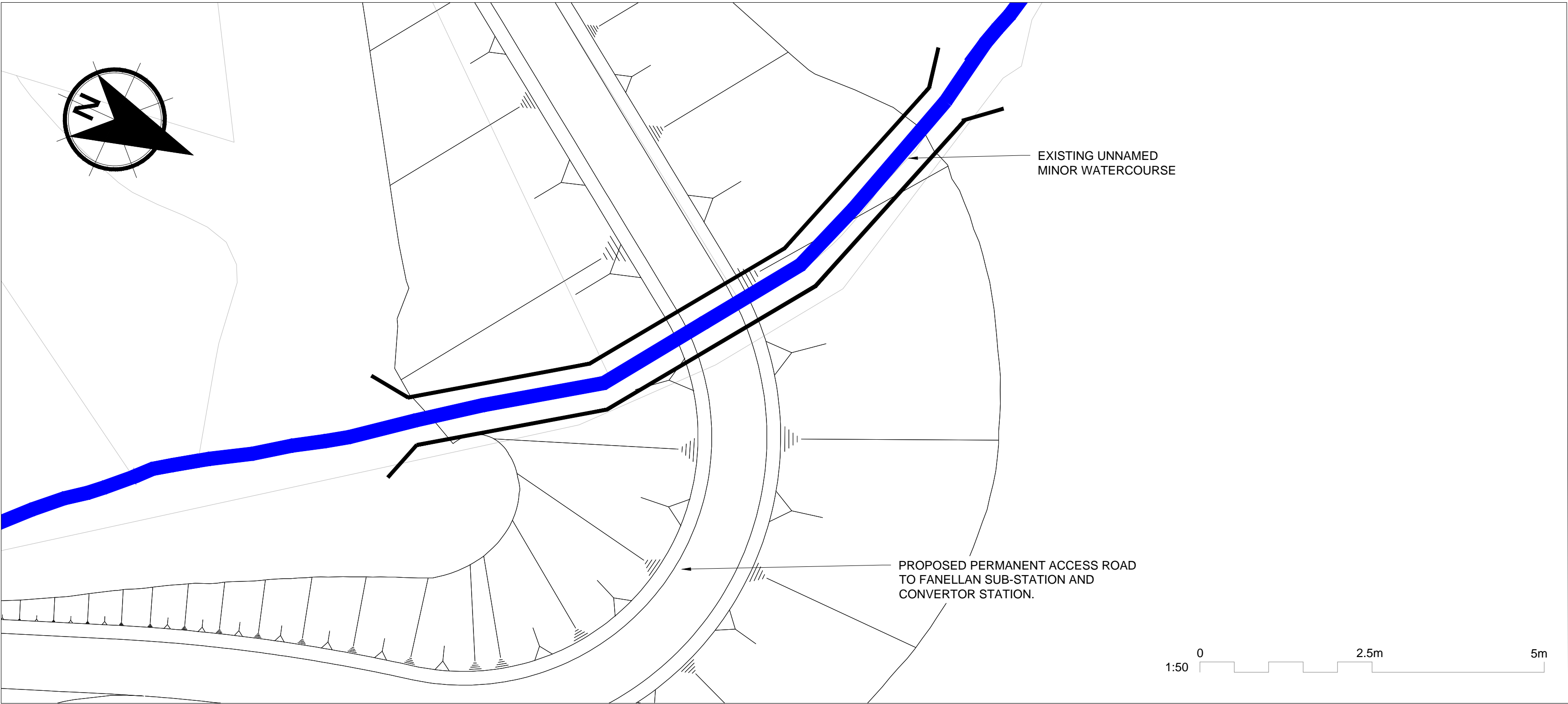
WATERCOURSE CROSSING LOCATION UNDER ACCESS ROAD
