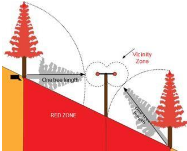
Plate 1.1: FISA 804 Tree Length and Red Zone (for a wood pole)
