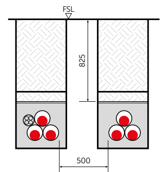
Typical double circuit cable arrangement
