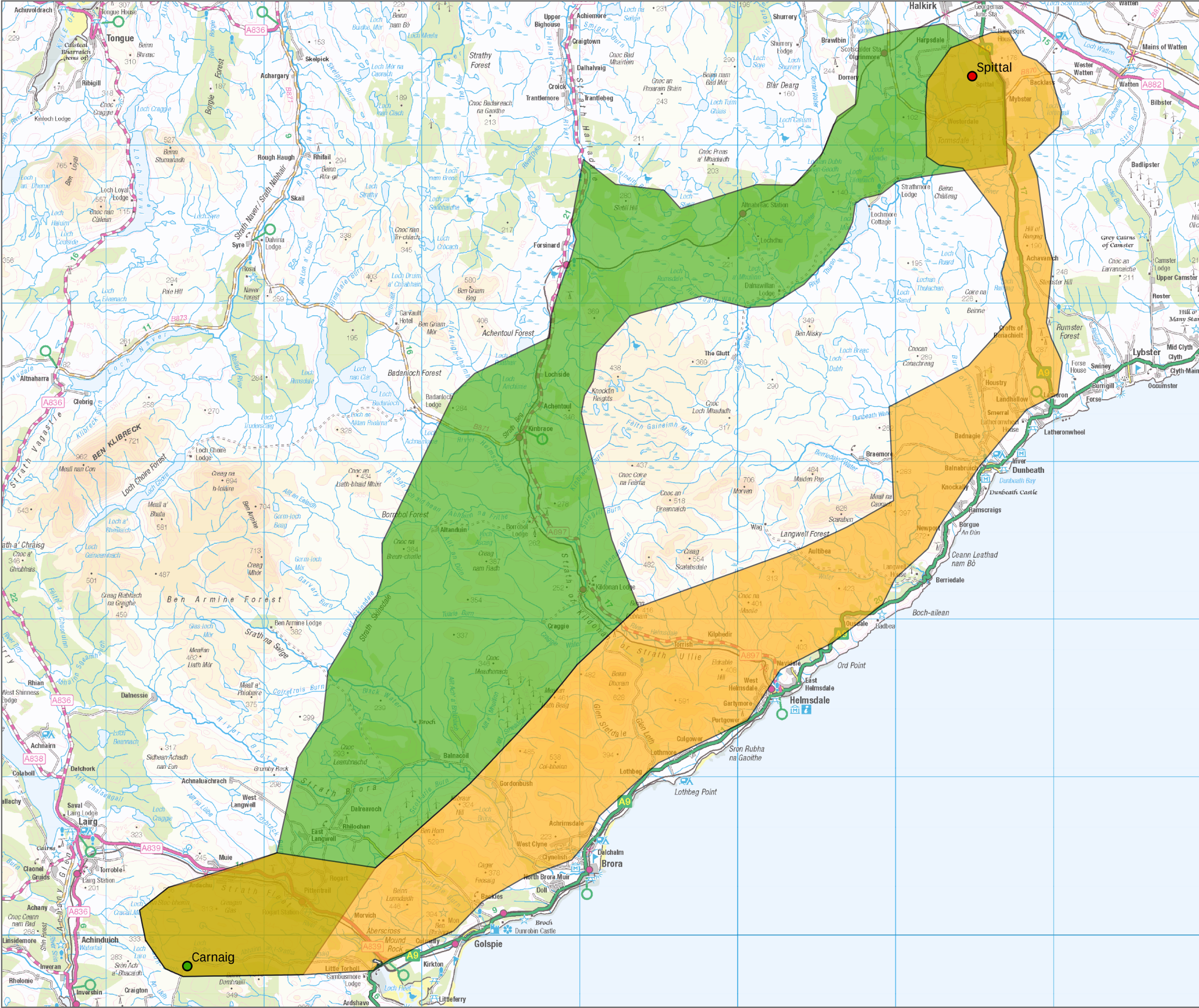
Figure 4.1 - 1 Spittal - Loch Buidhe - Beauly 400 kV OHL Connection Corridor Options
