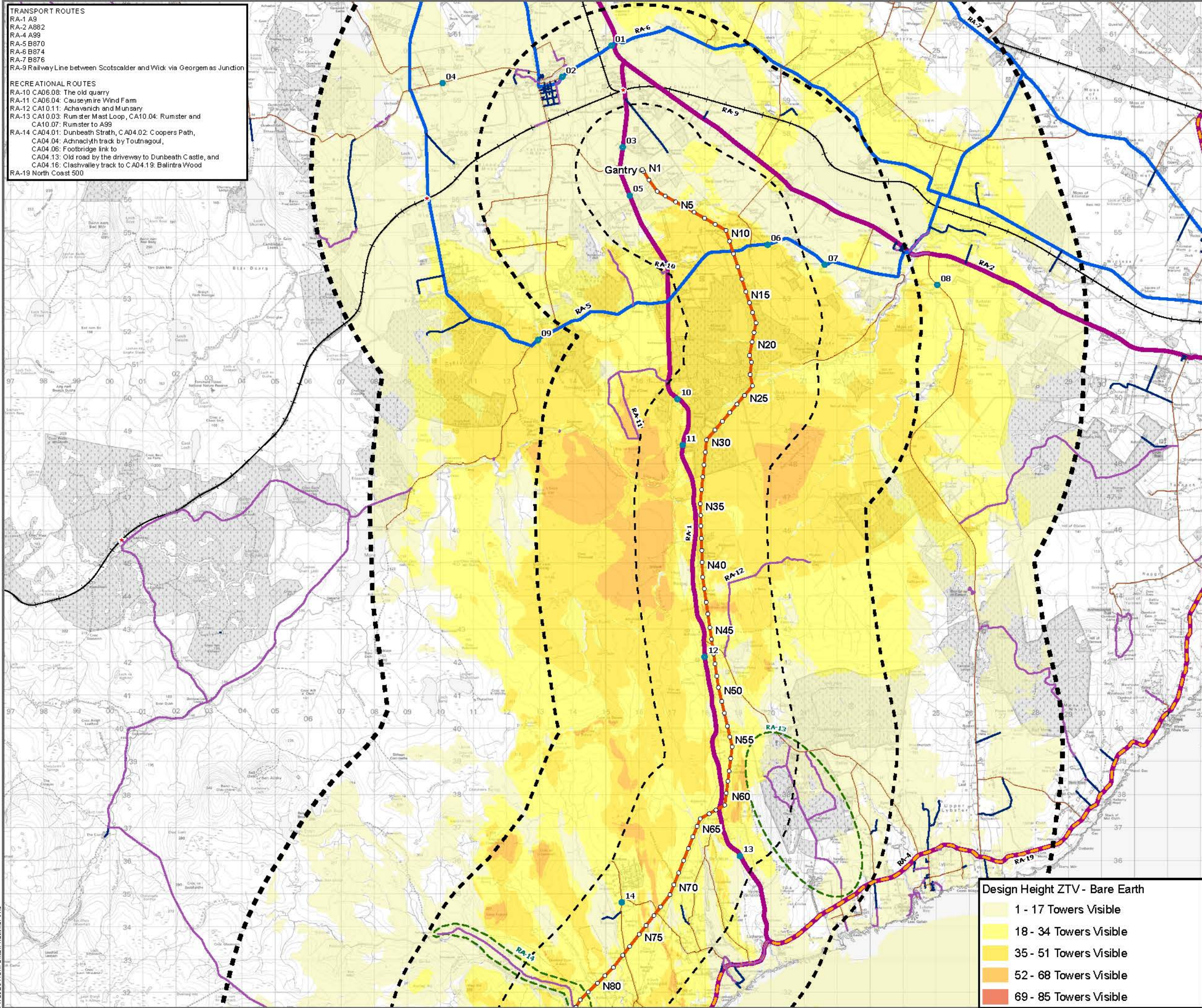
Figure 7.4 - 3 Spittal - Loch Buidhe - Beaully 400 kV OHL Connection Visual Receptors Section A (North)
