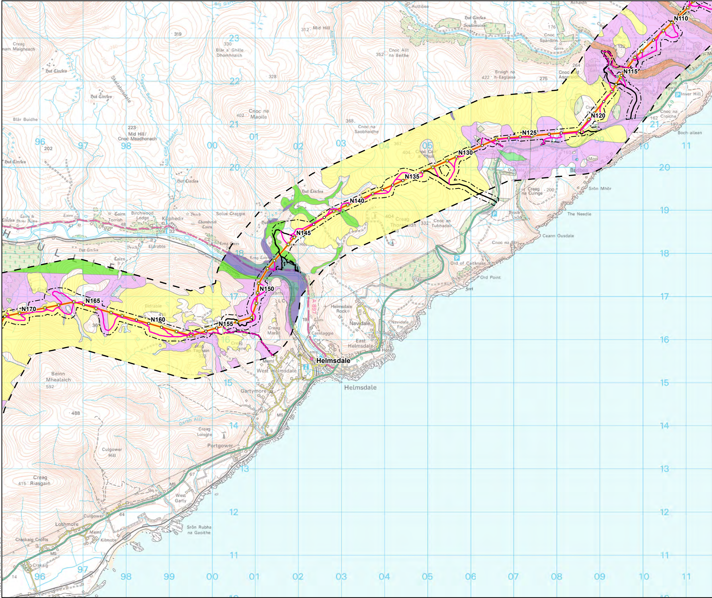
Figure 11.1 - 4 Spittal - Loch Buidhe - Beauly 400 kV OHL Connection Superficial Geology
