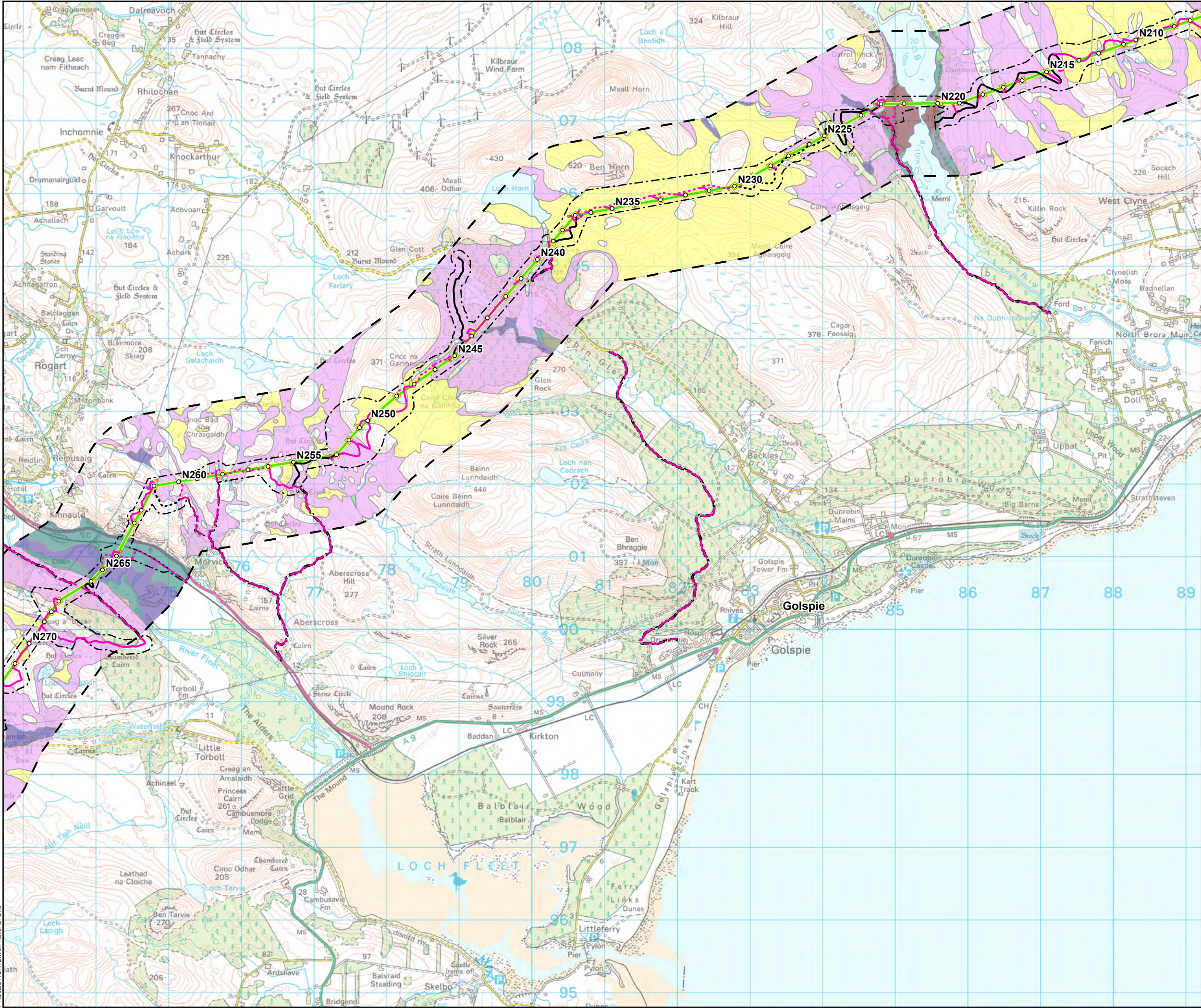
Figure 11.1 - 6 Spittal - Loch Buidhe - Beaully 400 kV OHL Connection Superficial Geology
