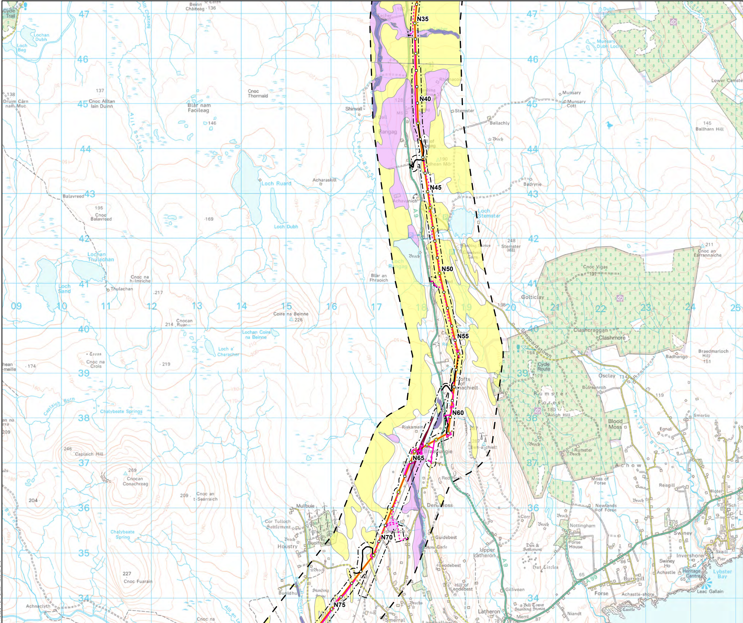
Figure 11.1 - 2 Spittal - Loch Buidhe - Beauly 400 kV OHL Connection Superficial Geology
