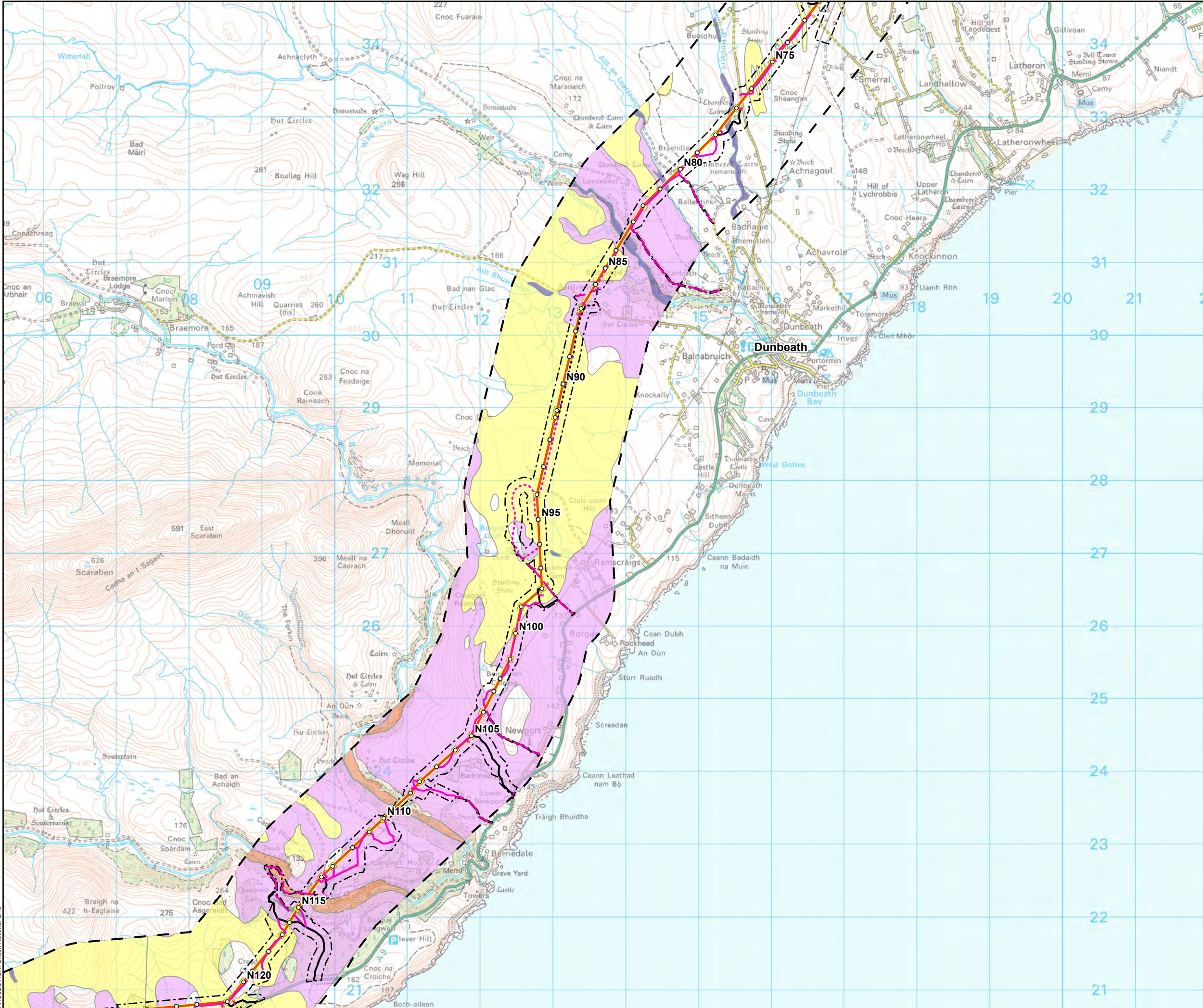
Figure 11.1 - 3 Spittal - Loch Buidhe - Beauly 400 kV OHL Connection Superficial Geology
