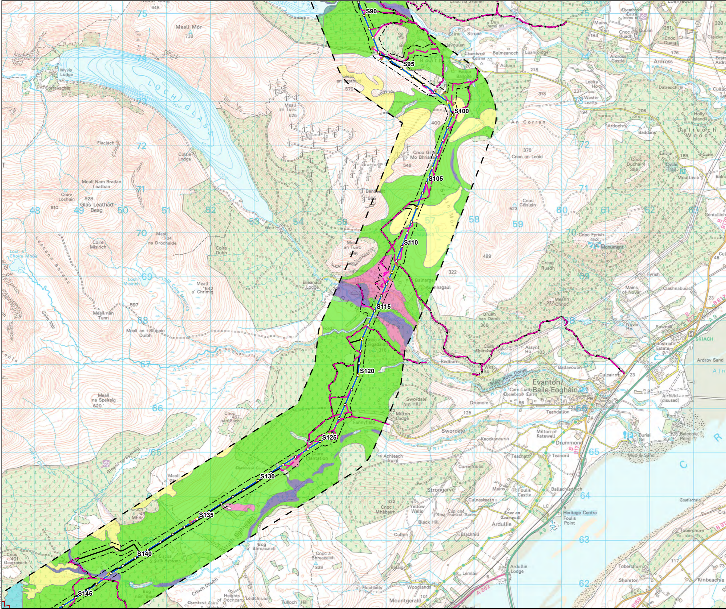
Figure 11.1 - 10 Spittal - Loch Buidhe - Beaulieu 400 kV OHL Connection Superficial Geology
