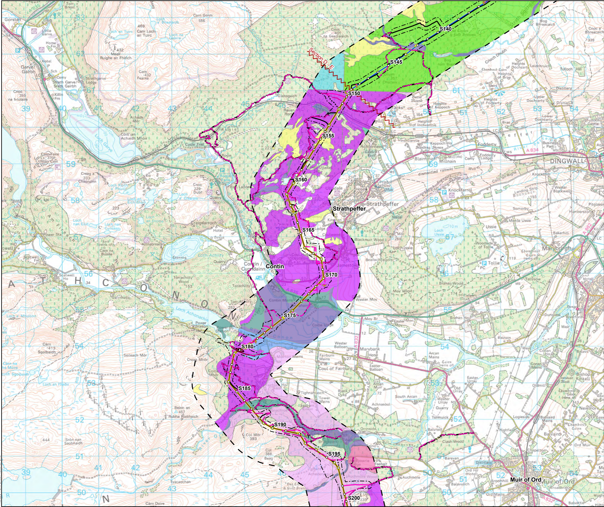
Figure 11.1 - 11 Spittal - Loch Buidhe - Beauly 400 kV OHL Connection Superficial Geology
