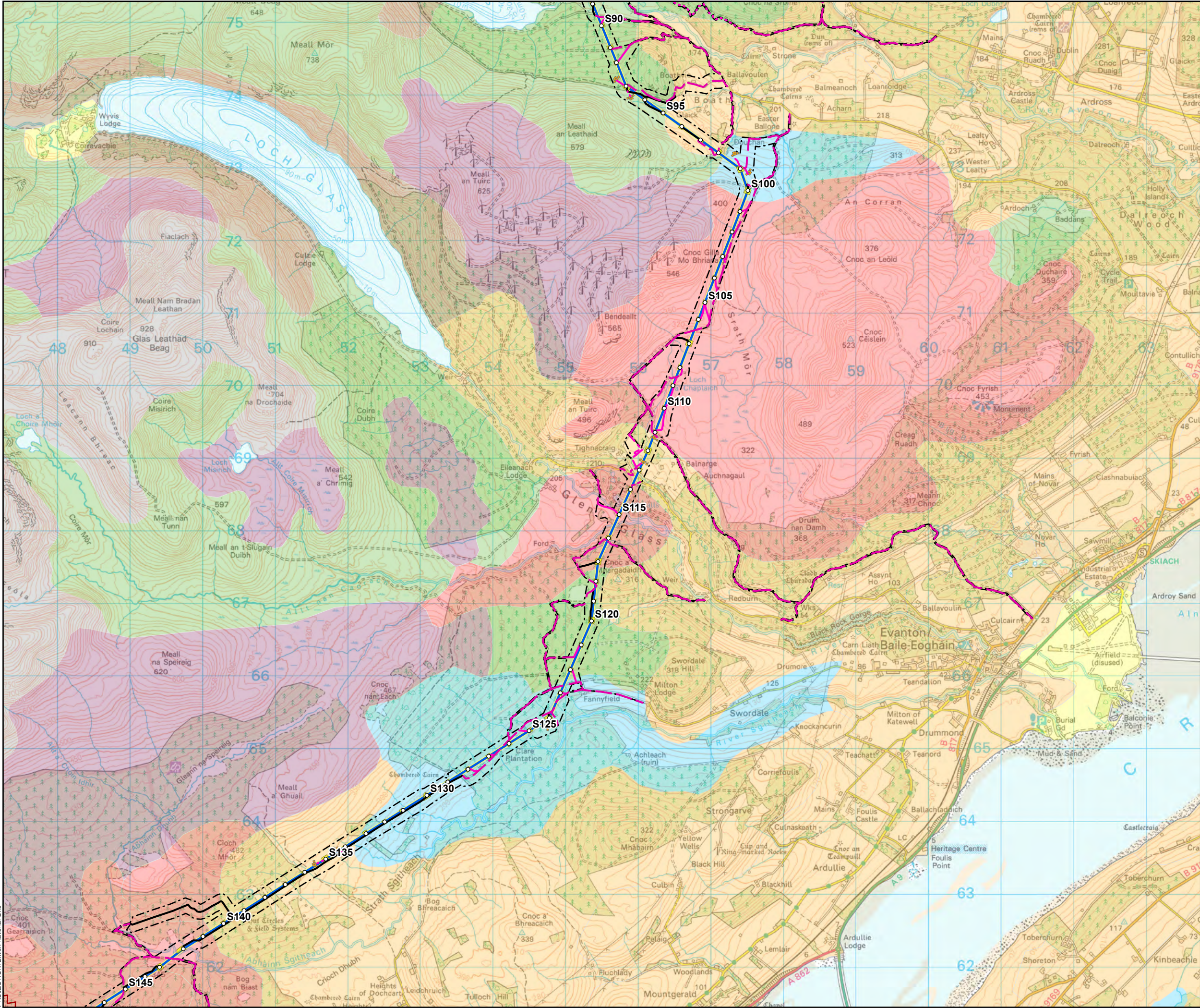
Figure 11.3 - 10 Spittal - Loch Buidhe - Beauly 400 kV OHL Connection National Soil Map of Scotland
