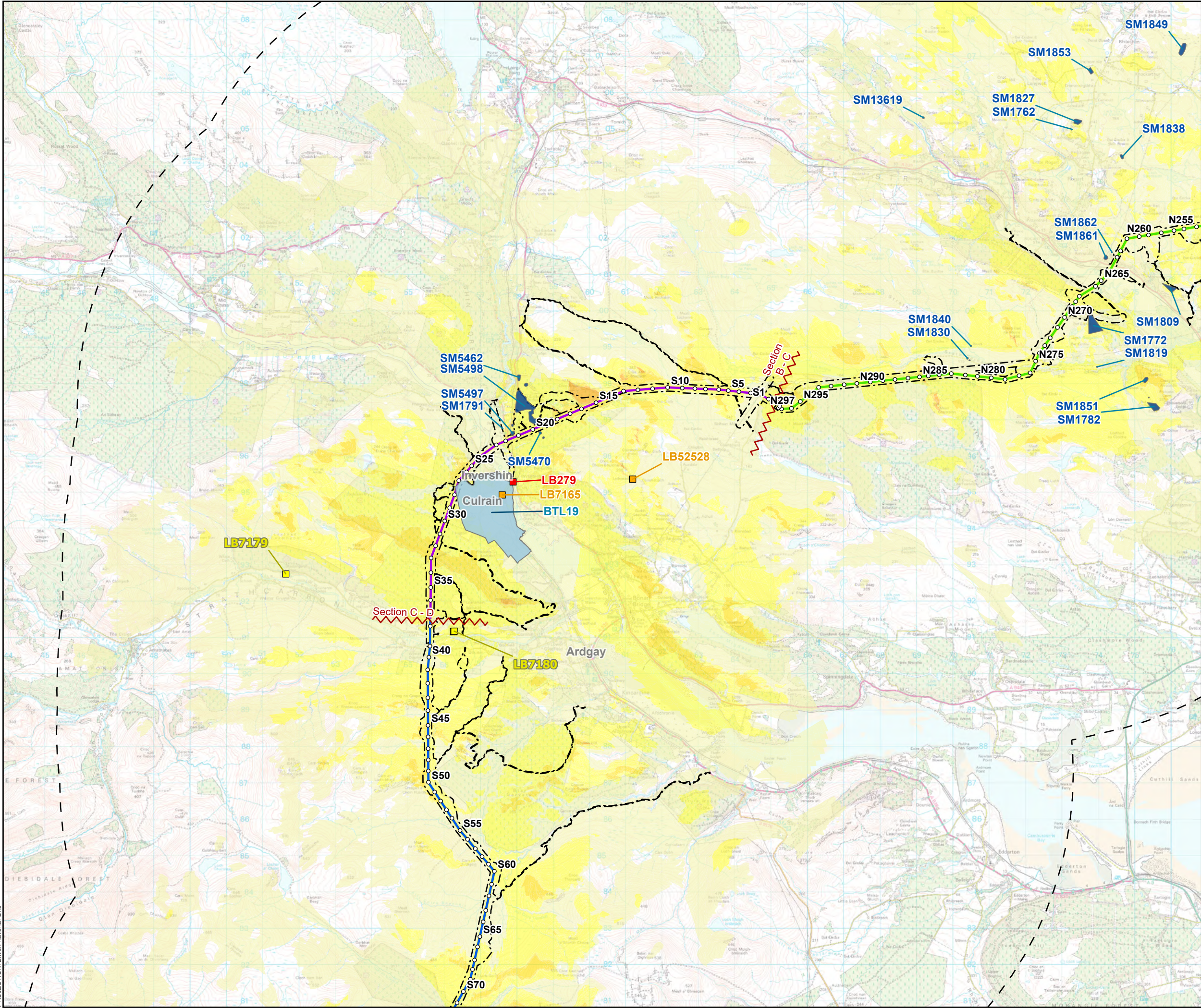
Figure 12.5 - 5 Spittal - Loch Buidhe - Beaulie 400 kV OHL Connection Sieved Setting Assets with ZTV (design height, bare earth)
