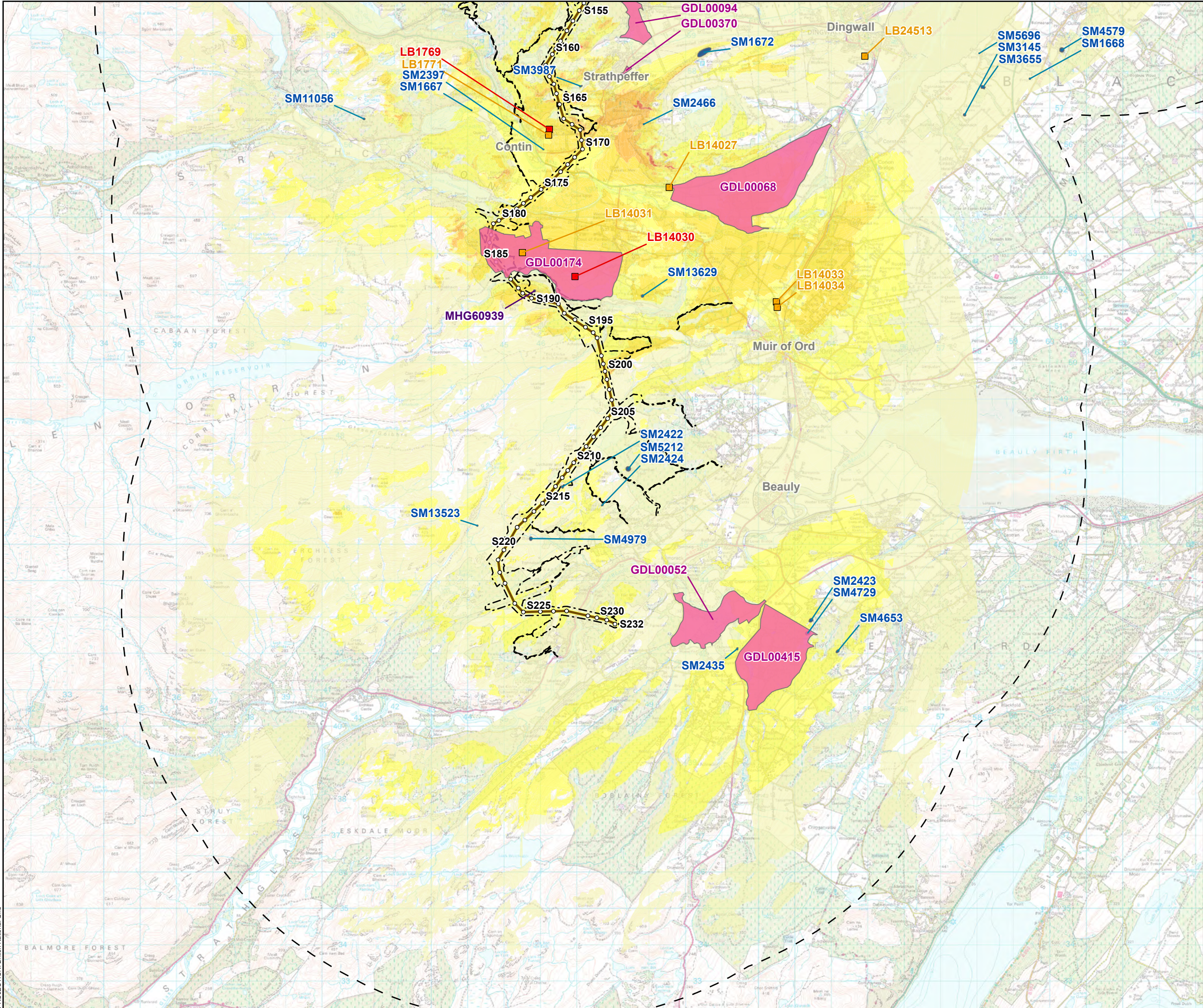
Figure 12.5 - 7 Spittal - Loch Buidhe - Beaulieu 400 kV OHL Connection Sieved Setting Assets with ZTV (design height, bare earth)
