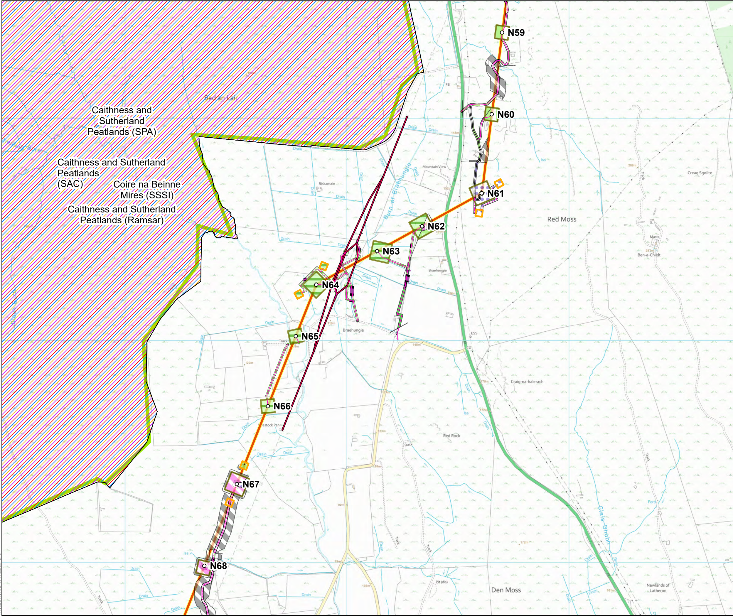
Figure 1: 9 Spittal - Loch Buidhe - Beaully 400 kV OHL Connection Baseline UK Habitat Classifications and Infrastructure included in the Biodiversity Net Gain Assessment
