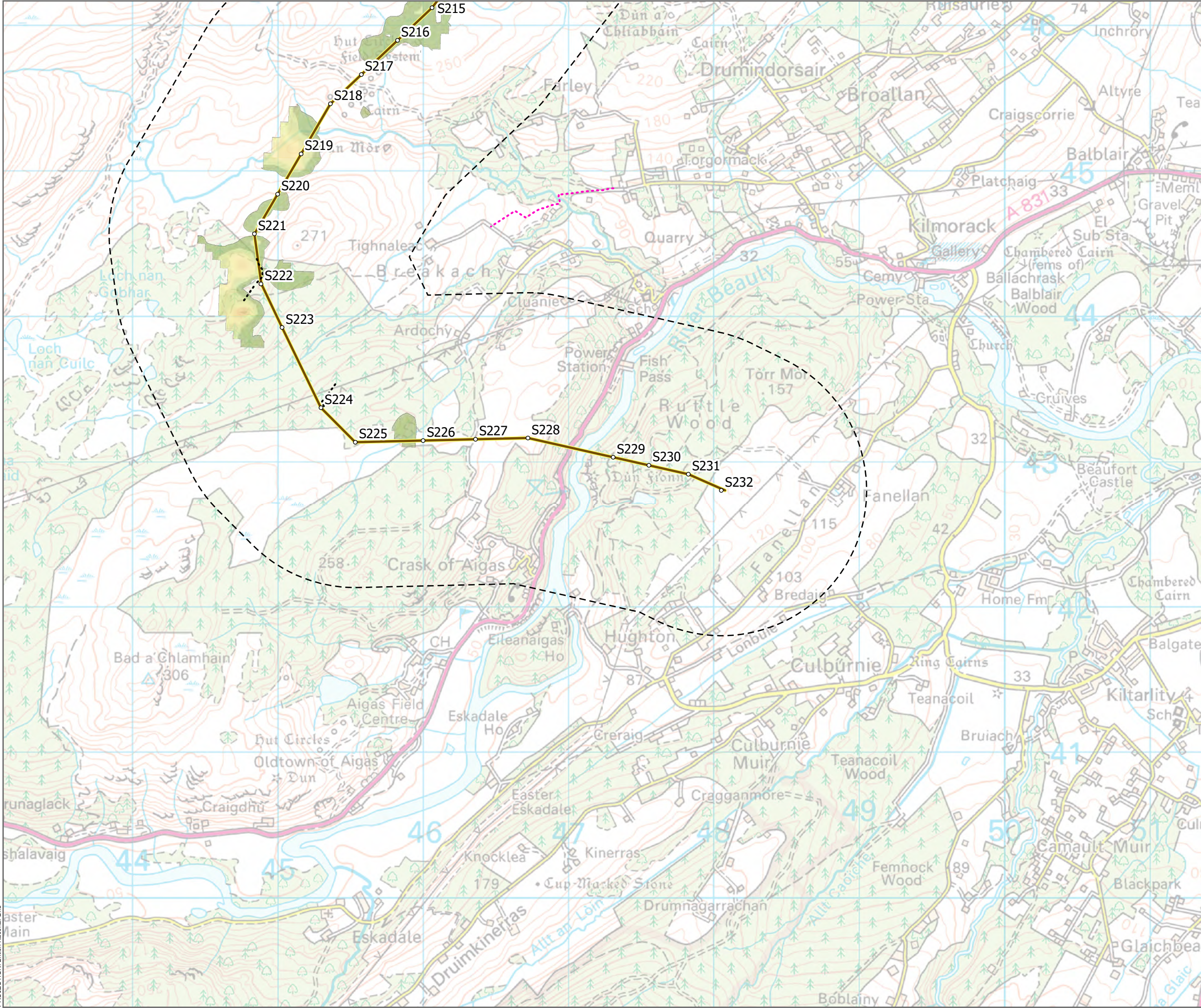
Figure 8 - 30 Spittal - Loch Buidhe - Beaulieu 400 kV OHL Connection Peat Landslide Hazard Risk Assessment Floating Tracks (PLHRA)
