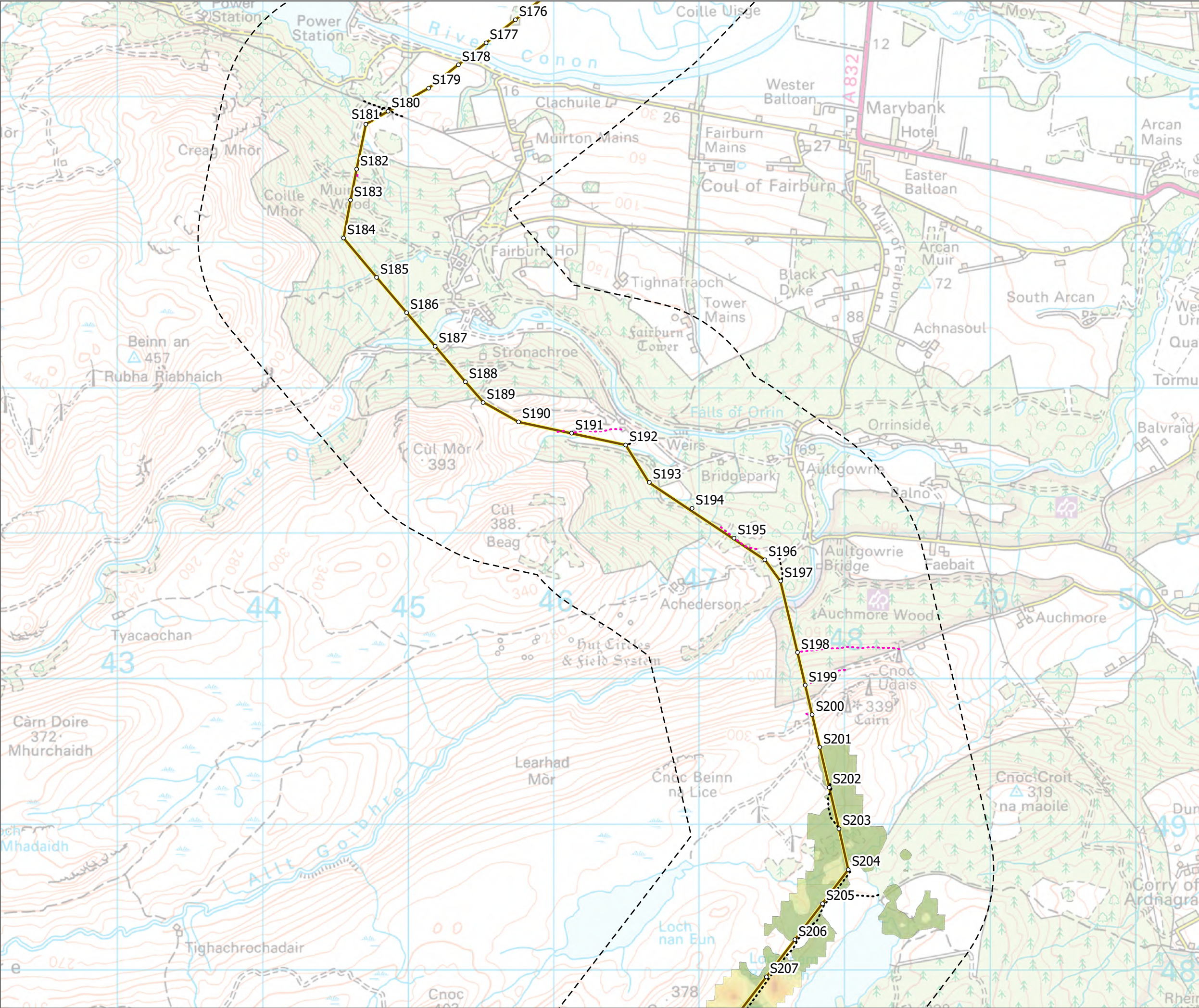
Figure 8 - 28 Spittal - Loch Buidhe - Beaully 400 kV OHL Connection Peat Landslide Hazard Risk Assessment Floating Tracks (PLHRA)
