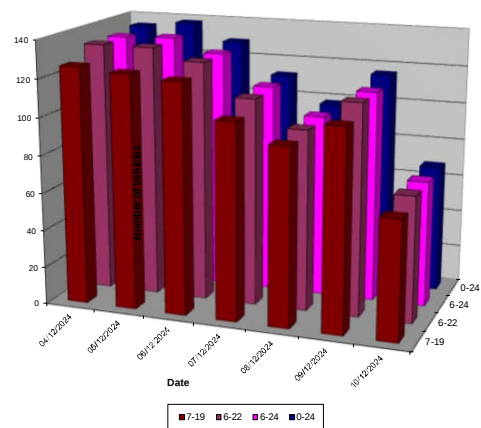
Vehicle Flow (Channel 2)
