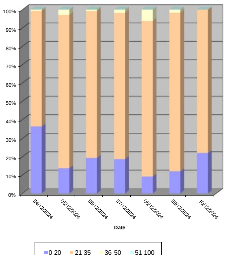
Speed Summary (MPH)
