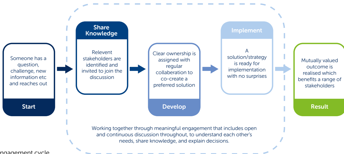
Figure 4: Engagement cycle
